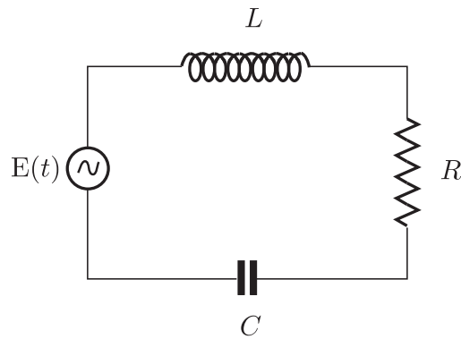
Figure 2.2.2 — Electric Circuit.
