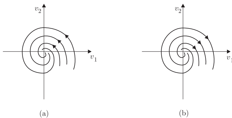
Figure 2.5.2 — Qualitative behavior of the dynamic response: (a) stable and (b) unstable focus.
