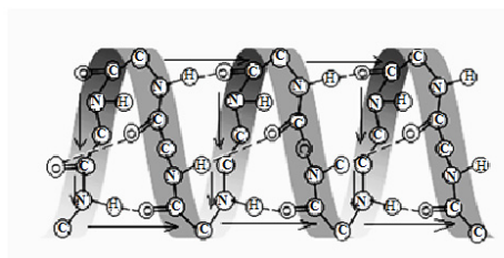
FIGURE 1. Scheme of the \alpha -helix structure in a typical protein.
